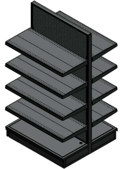
3ft x 66" tall double-sided gondola fixture shown with (8) steel shelves
