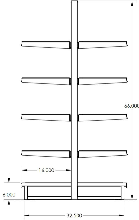
3ft x 66" tall double-sided gondola fixture shown with (8) steel shelves
